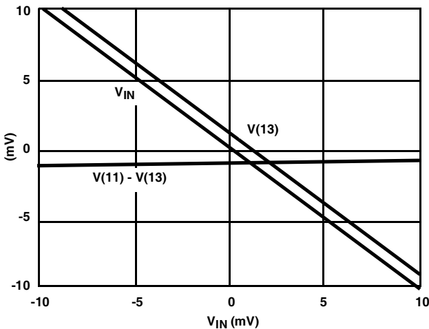
FIGURE 8. HA5024 INPUT OFFSET VOLTAGE
