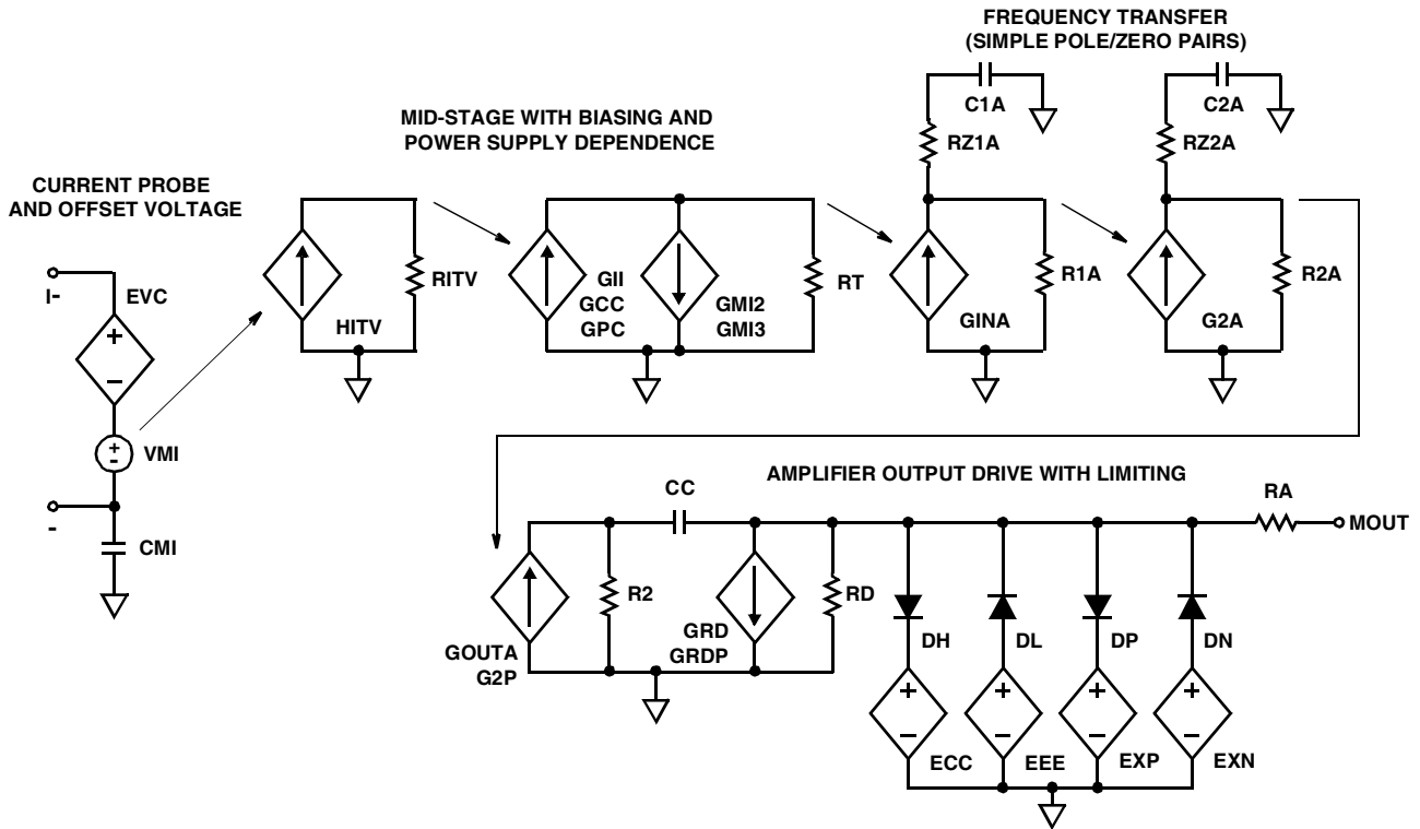
FIGURE 1B. HA5024 MACROMODEL OUTPUT STAGE
