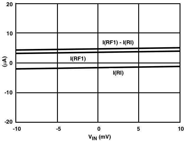
FIGURE 7. HA5024 INPUT CURRENT
