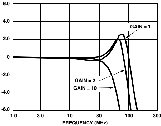
FIGURE 2. HA5024 NON-INVERTING OP AMP AC TRANSFER FUNCTION
