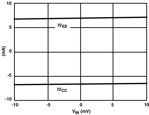
FIGURE 6. HA5024 POWER SUPPLY CURRENT DRAIN PER AMPLIFIER
