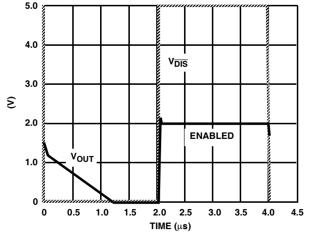
FIGURE 9. HA5024 ENABLE/DISABLE RESPONSE TIME
