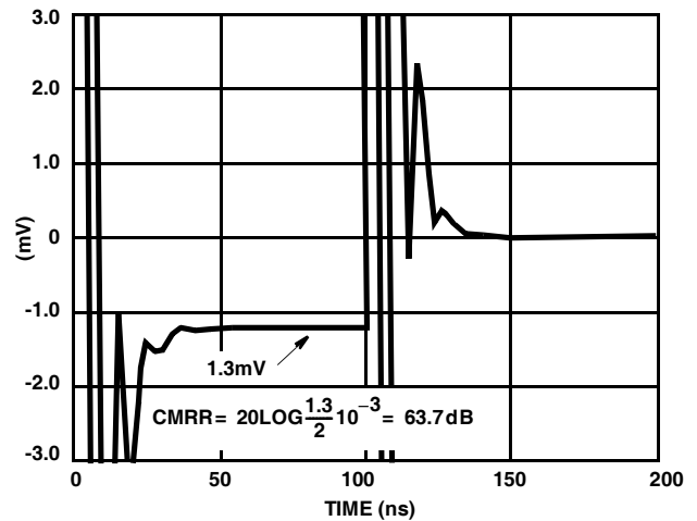
FIGURE 5. HA5024 CMRR
