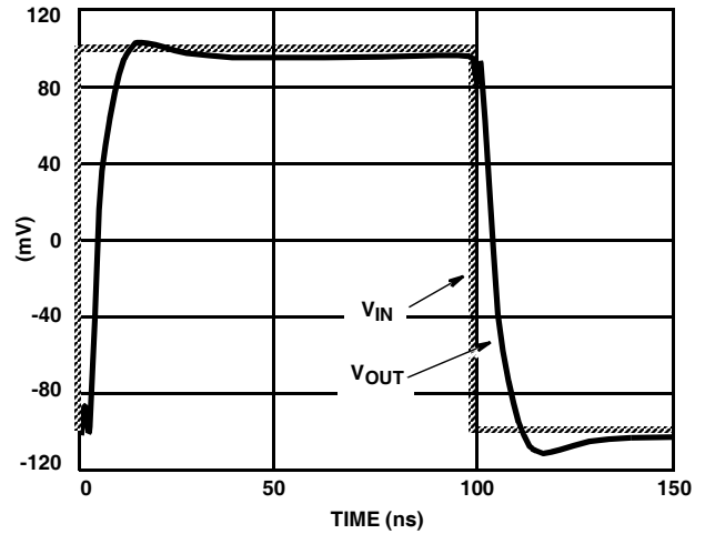
FIGURE 4. HA5024 SMALL SIGNAL PULSE RESPONSE
