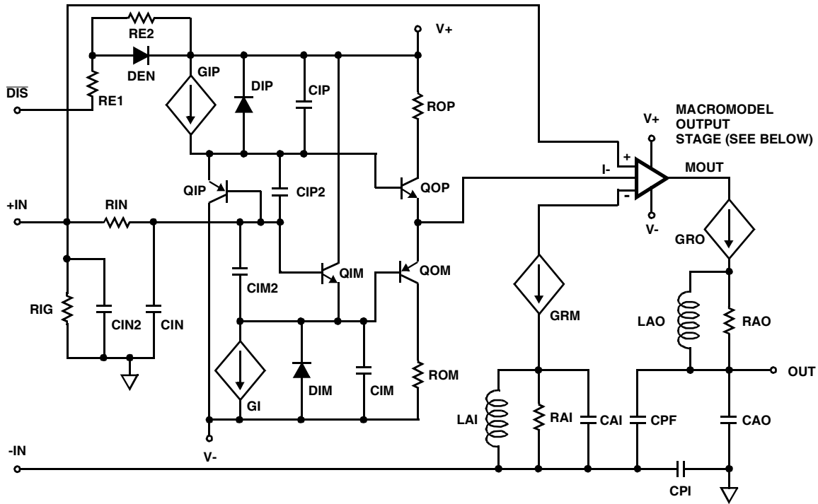
FIGURE 1A. HA5024 AMPLIFIER MACROMODEL SCHEMATIC
